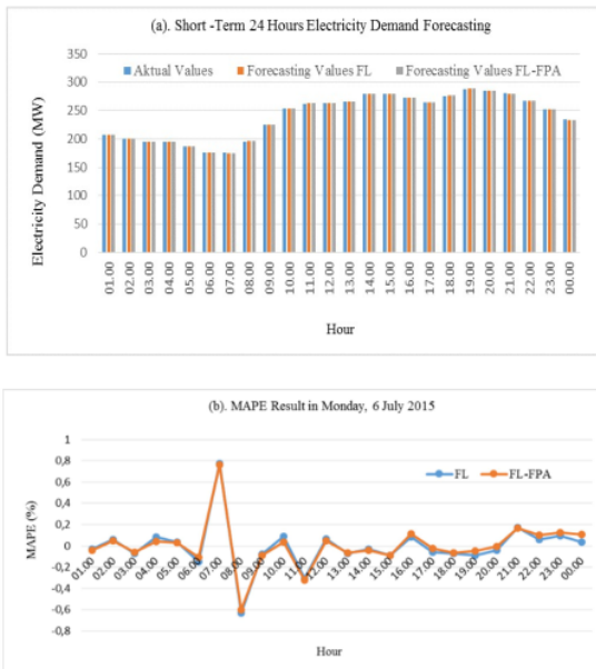
Figure 2 (a)(b).Short-term load forecasting results and MAPE values for FL and FL-FPA methods.
